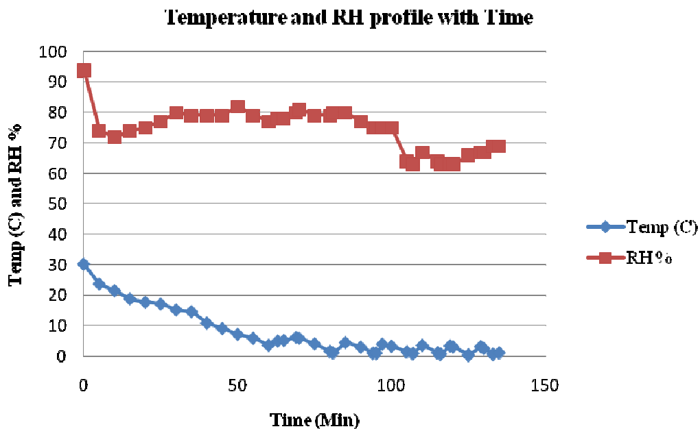
Fig. 4. Temperature and relative humidity variation with time in the developed setup
