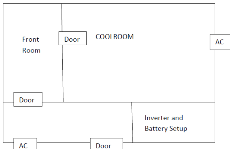
Fig.1. Cross Sectional View of the developed cold storage facility
